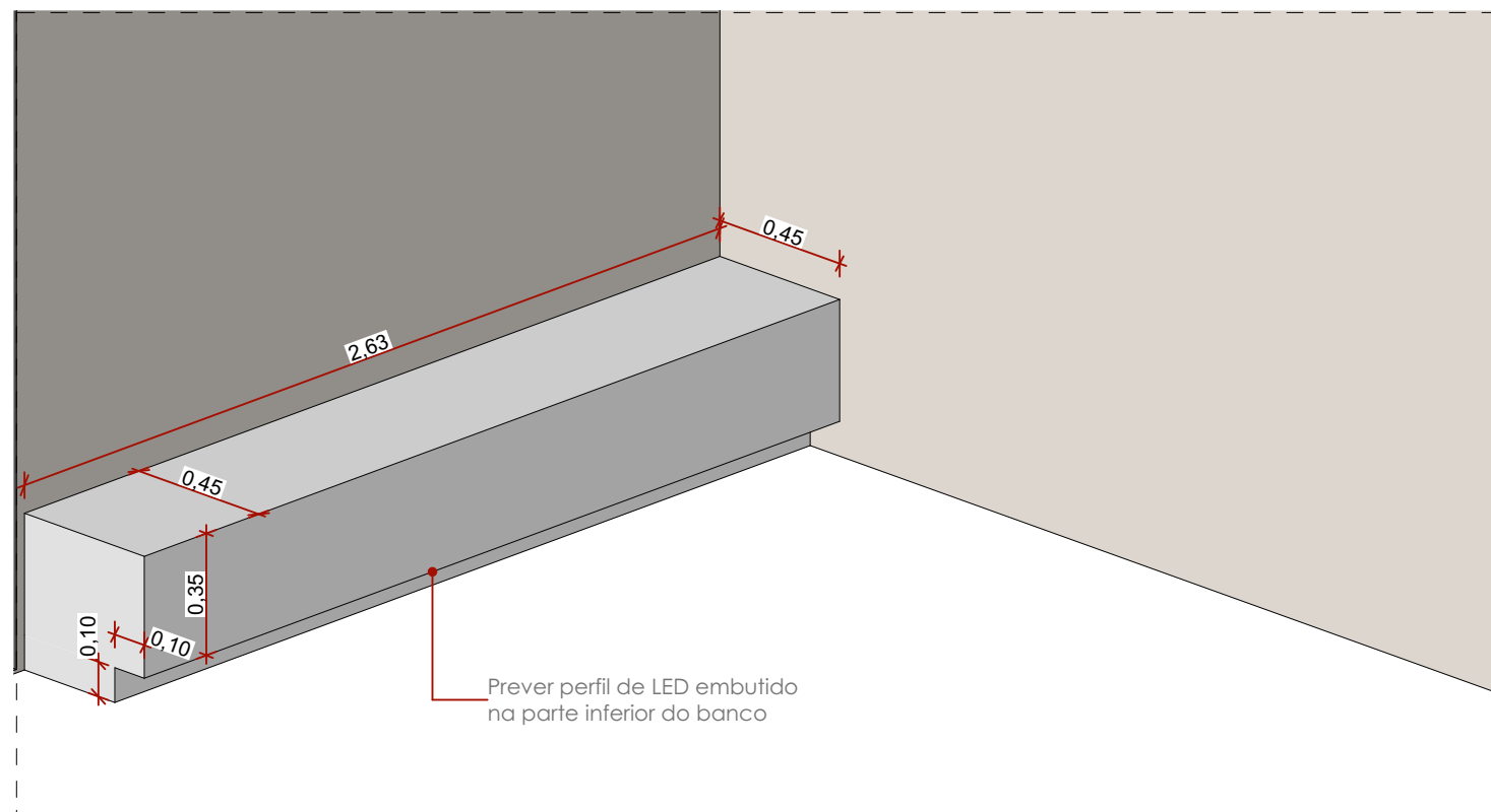
Def. Banco de alvenaria Sauna 1:25
